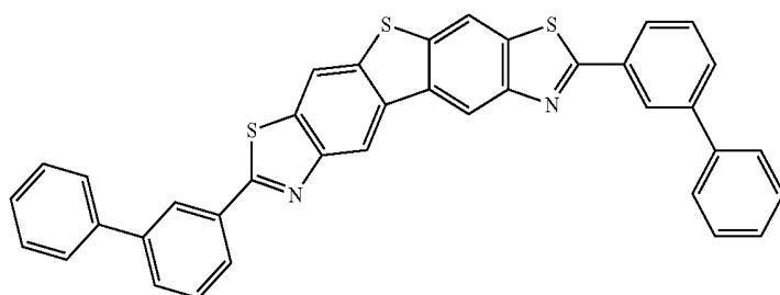
Compound 30
