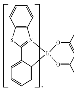
Ir(BT) 2 (acac)
