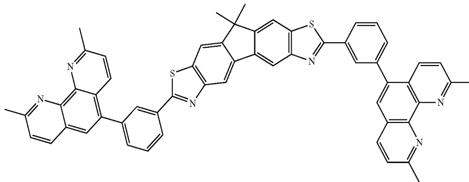
Compound 4
