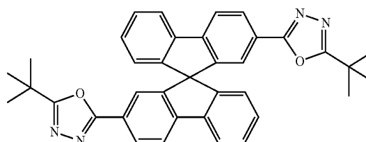
spiro-PBD
