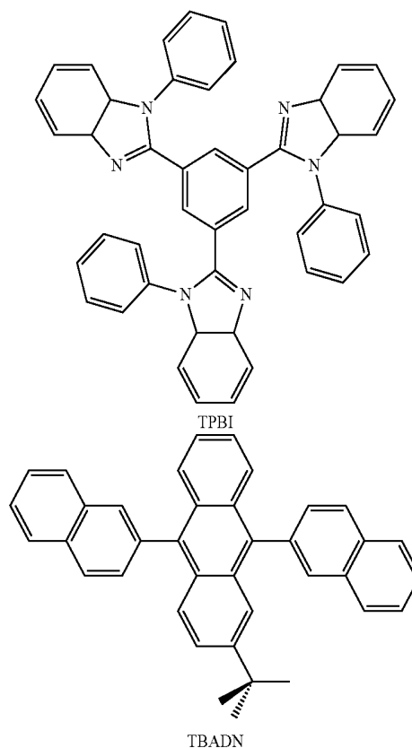
TBADN
