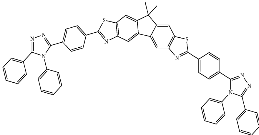
Compound 10
