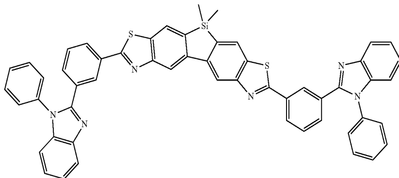
Compound 19
