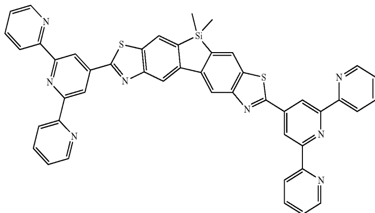
Compound 26
