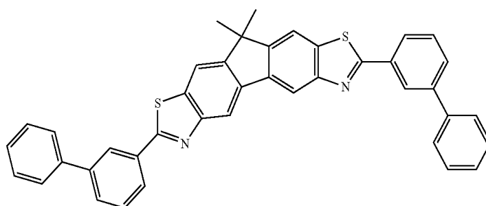
Compound 1
