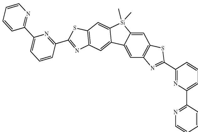
Compound 23
