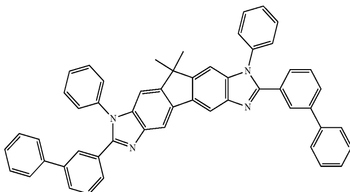
Compound 31
