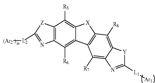
Formula 1
