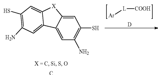
Compound 1
