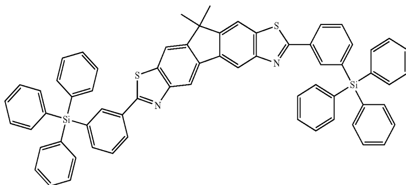
Compound 6
